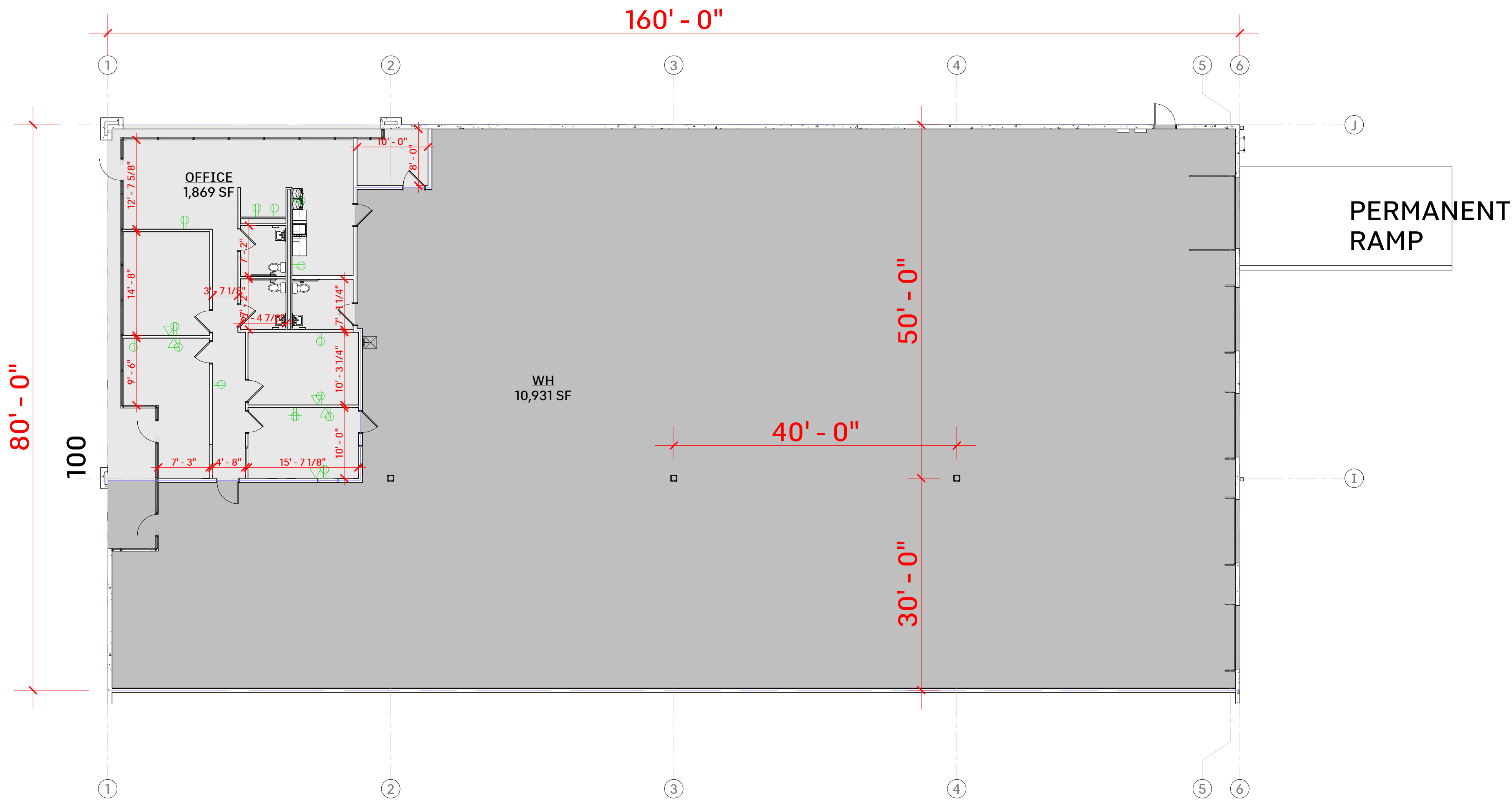
KEY PLAN
